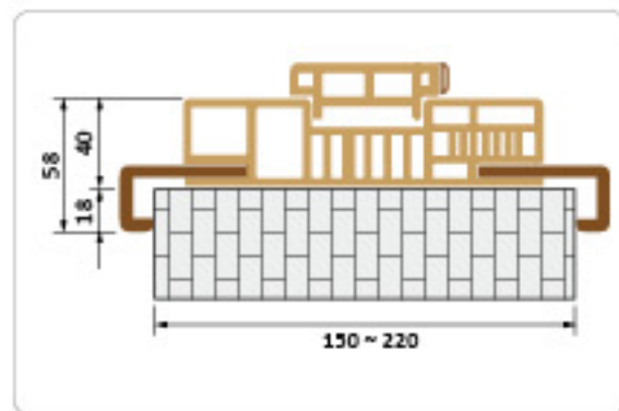
C1655 嵌入雙線板
